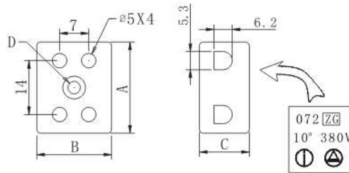
072 陶瓷接線座 CERAMIC WIRE CONNECTOR SET
